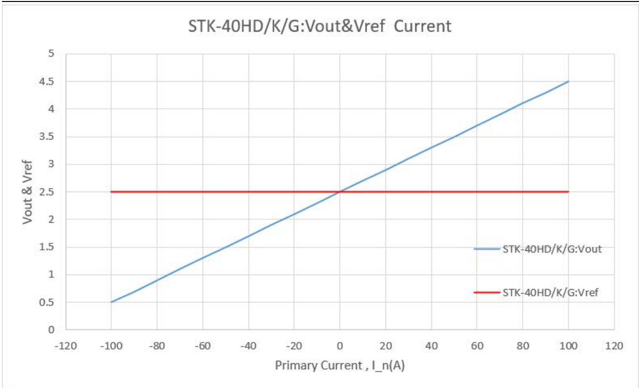
The dependence of Vout&Vref of STK-40HD-K/G on the primary current.
