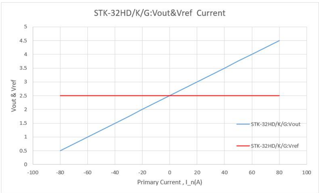
The dependence of Vout&Vref of STK-32HD-K/G on the primary current.
