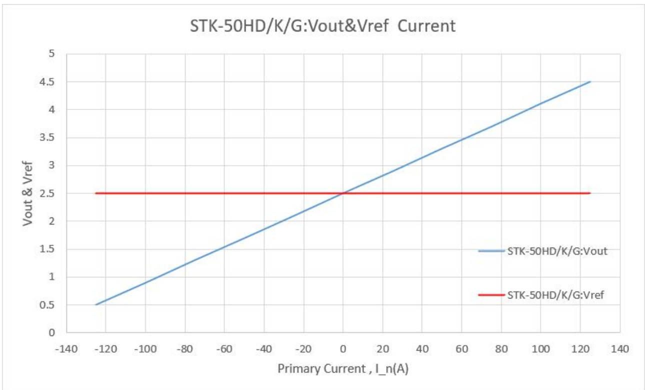
The dependence of Vout&Vref of STK-50HD-K/G on the primary current.
