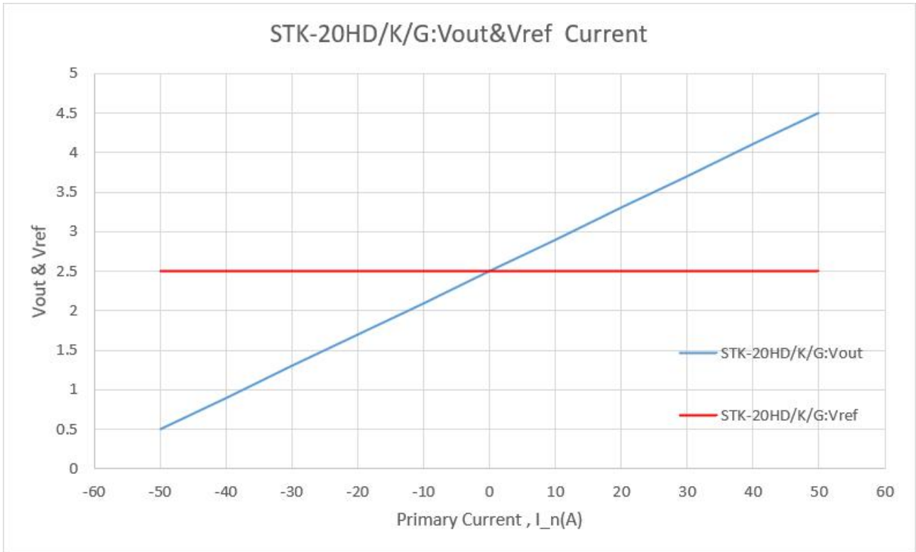
The dependence of Vout&Vref of STK-20HD-K/G on the primary current.
